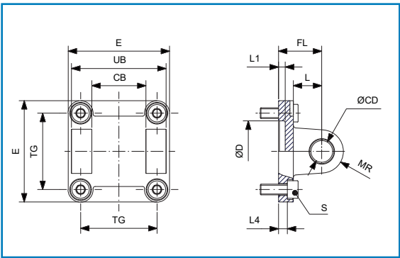
Cerniera femmina MP2 Female hinge MP2
